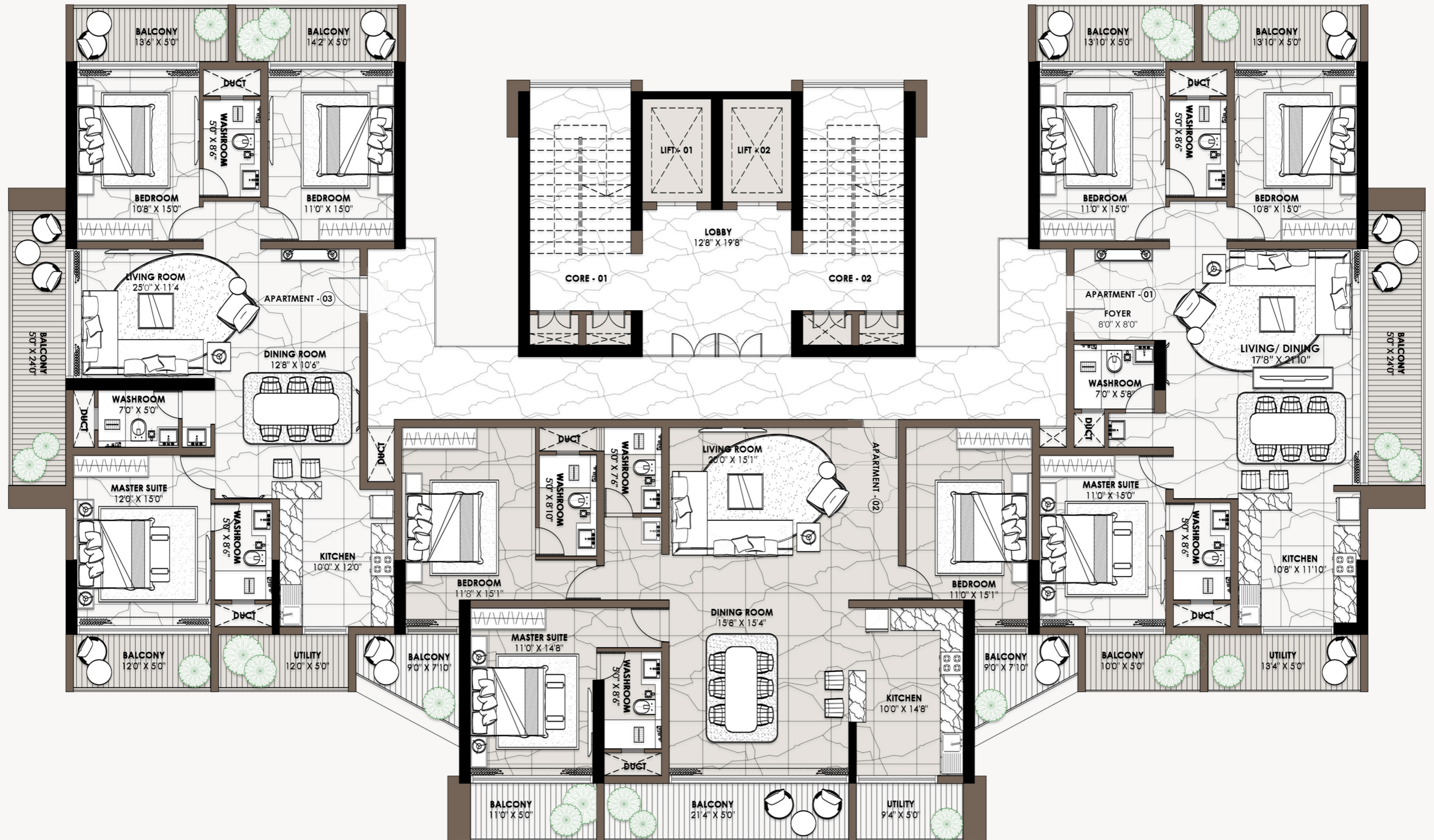
TYPICAL FLOOR PLAN
